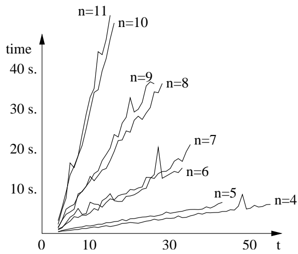
Figure 2: Performance in various dimensions
