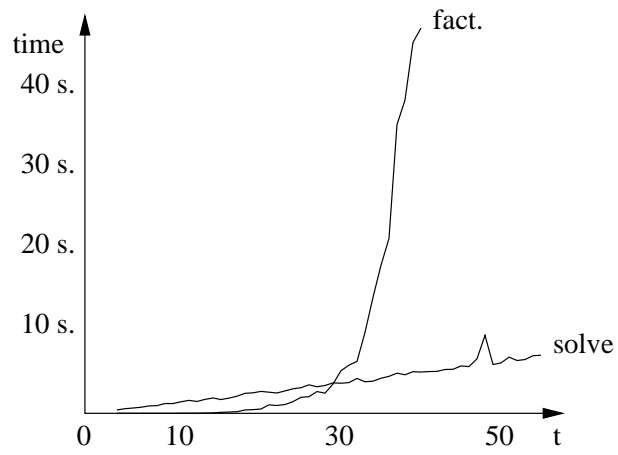
Figure 1: Performance in dimension 4
